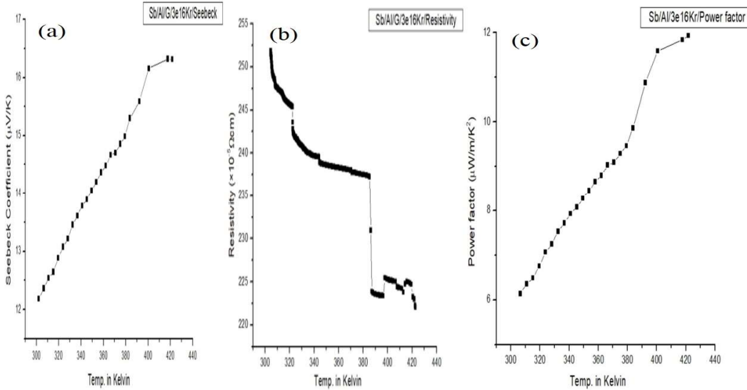
Fig 7 Graph of (a) Seebeck co-efficient, (b) Resistivity and (c) Power factor verses temperature for Kr irradiated sample`
