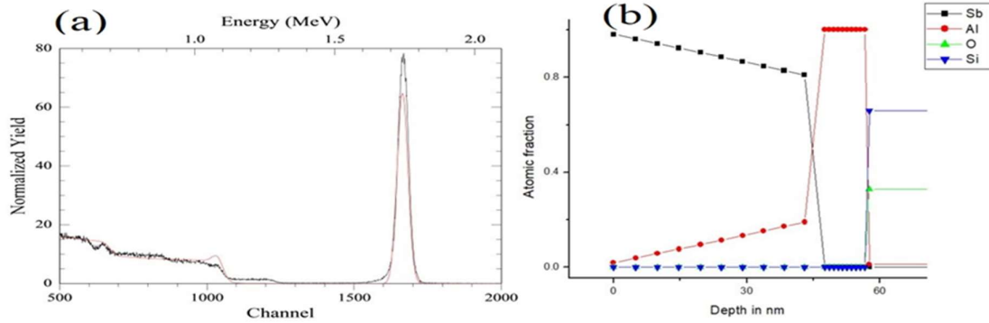
Fig 2 (a) RBS Spectra and (b) Depth profile of Pristine Sb/Al sample
