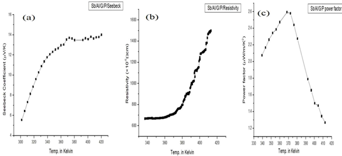
Fig 6 Graph of (a) Seebeck co-efficient, (b) Resistivity and (c) Power factor verses temperature for Pristine sample
