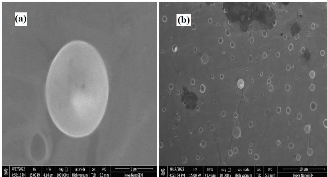
Fig 5 SEM of the Sb/Al Kr irradiated sample with magnification (a) 100Kx (b) 10Kx
